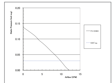
Performance Curve
