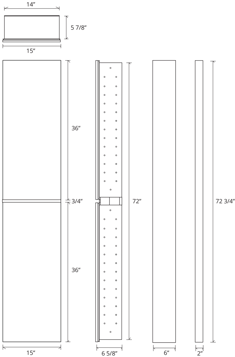
Side Mirror Kit SMK6-72 Order for Surface Mount Side Mirror Kit SRMK2-72 Order for Semi-Recessed Mount
