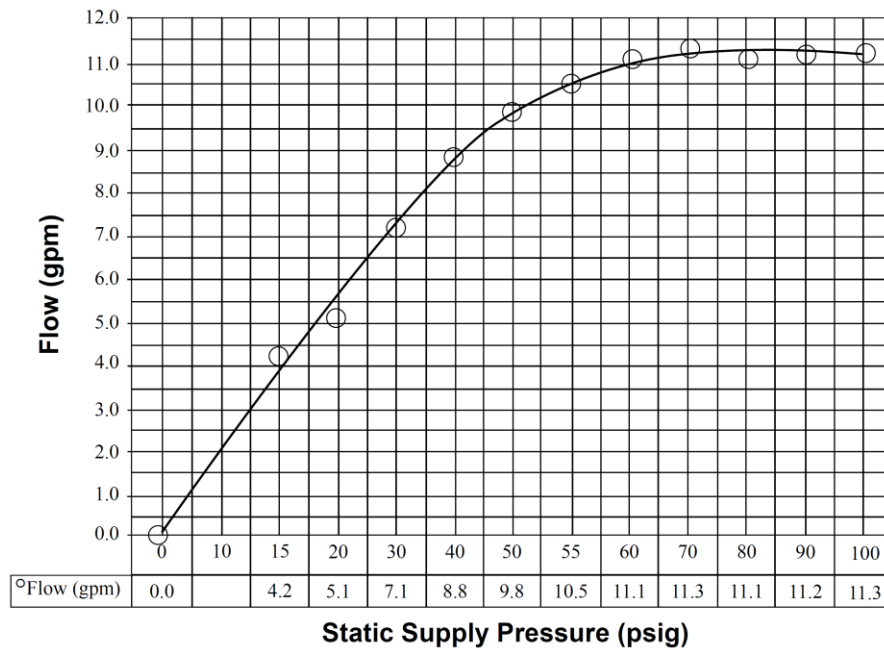
Flow Rate vs. Inlet Pressure
