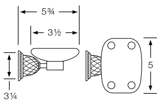
180-0.6/180-0.7 Tumbler Holder/Soap Dish (SV/TV)
