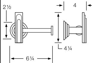
160-0.9A/B/C/D Mirror (SV)
