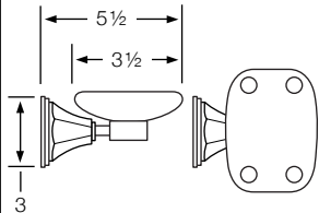
205-0.6-T6/205-0.7-T6 Tumbler Holder/Soap Dish (SV/TV)
