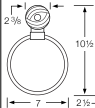
201-0.3 Towel Ring (FV/SV)
