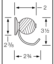
201-0.9A/B/C/D Mirror (SV)
