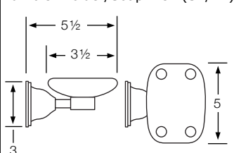
205-0.6-T7/205-0.7-T7 Tumbler Holder/Soap Dish (SV/TV)
