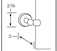
201-0.9A/B/C/D Mirror (SV)
