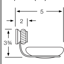
316-0.7 Soap Dish (SV)
