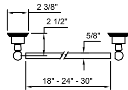
Towel Bar - Top View
