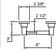
Toilet Paper - Top View
