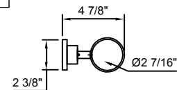
Soap Dish / Tooth Brush Holder - Side View
