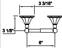
Toilet Paper - Top View
