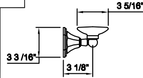
Soap Dish / Tooth Brush Holder - Side View
