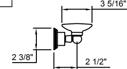
Soap Dish / Tooth Brush Holder - Side View
