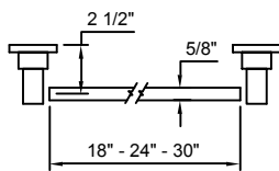
Towel Bar - Top View
