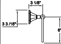
Towel Ring - Side View
