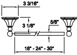
Towel Bar - Top View
