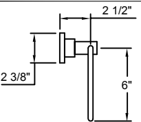
Towel Ring - Side View
