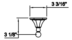
Robe Hook - Top View
