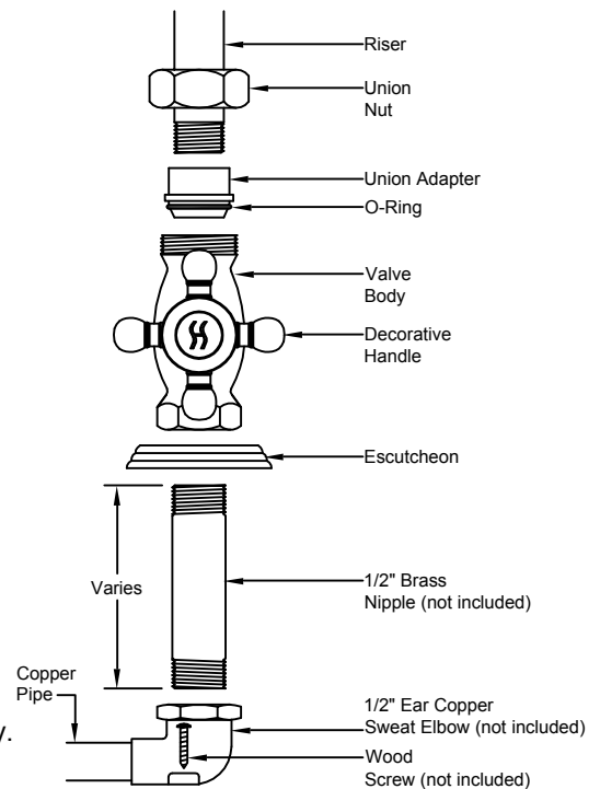
Exploded View
