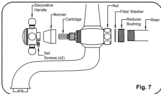
Exploded View
