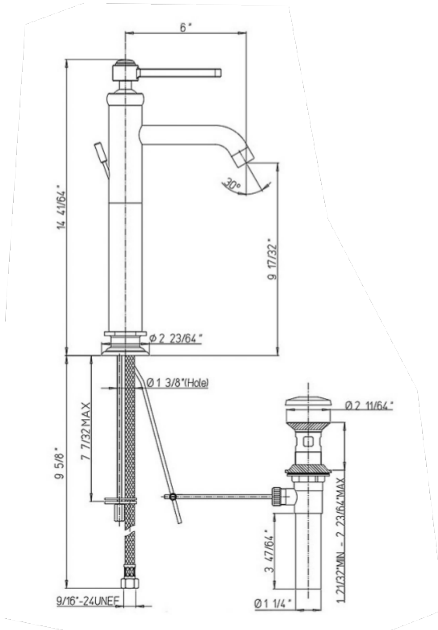
Firenze tall single lever handle lavatory vessel
