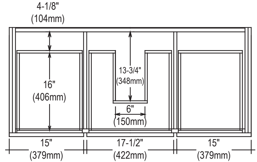
4. Side view line drawing
