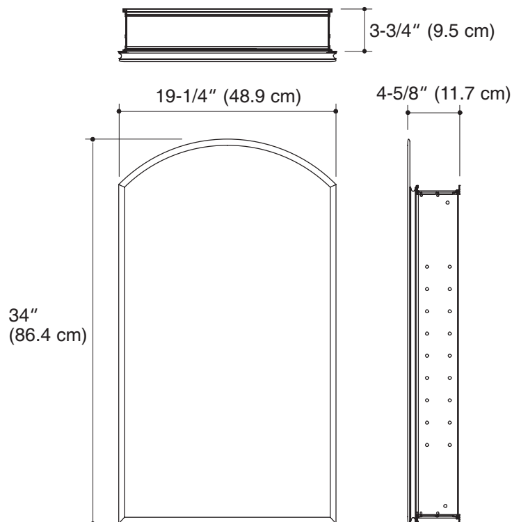
Product Diagram
