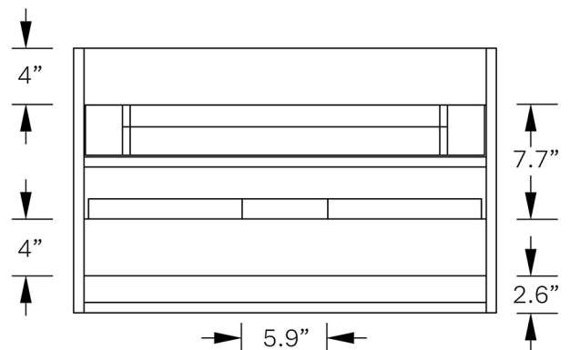
FCB4124 Cabinet Back
