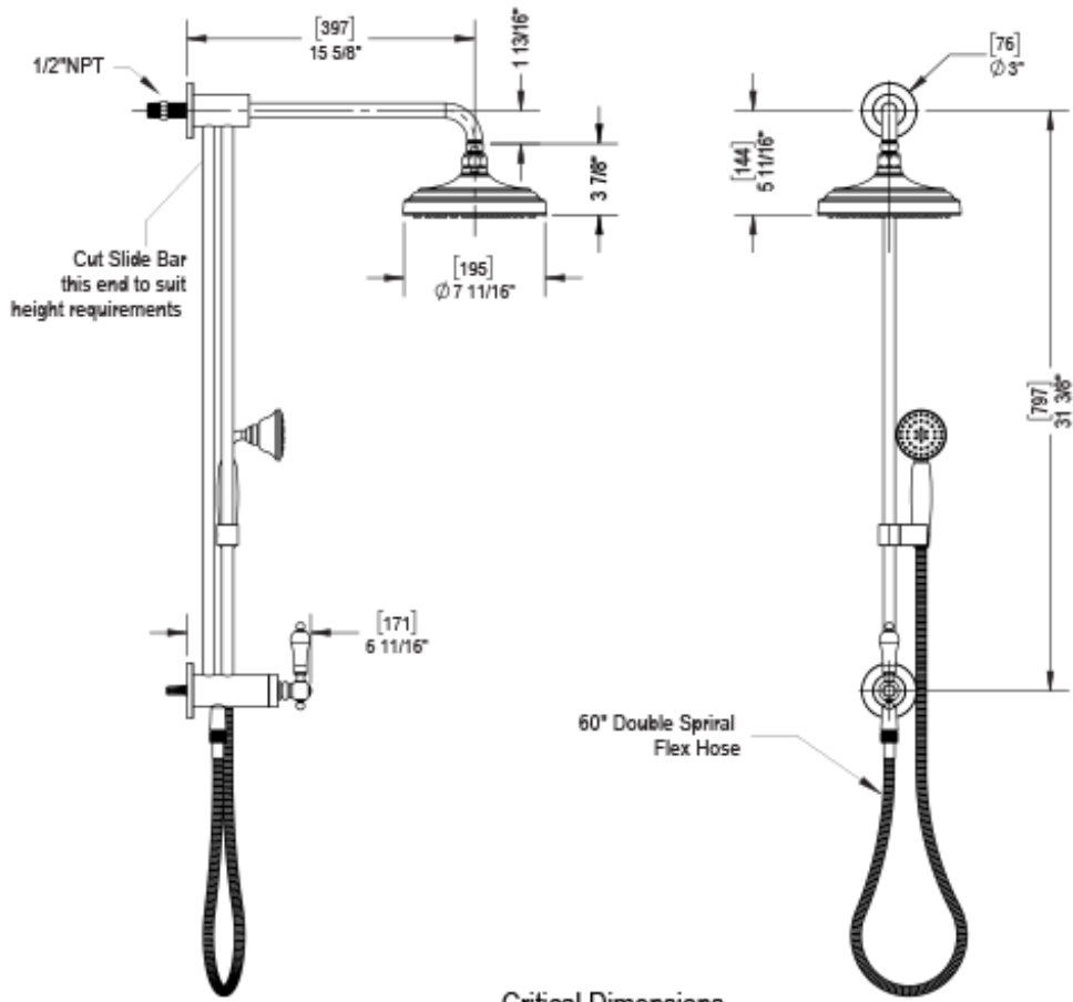
Critical Dimensions
