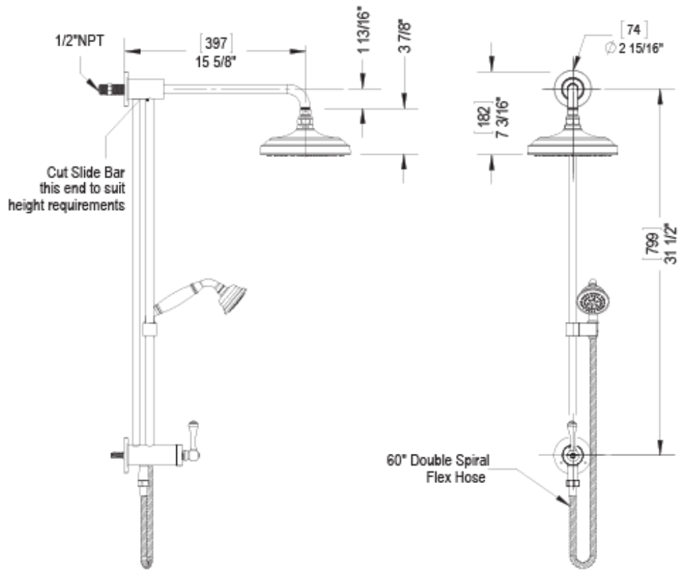
Critical Dimensions
