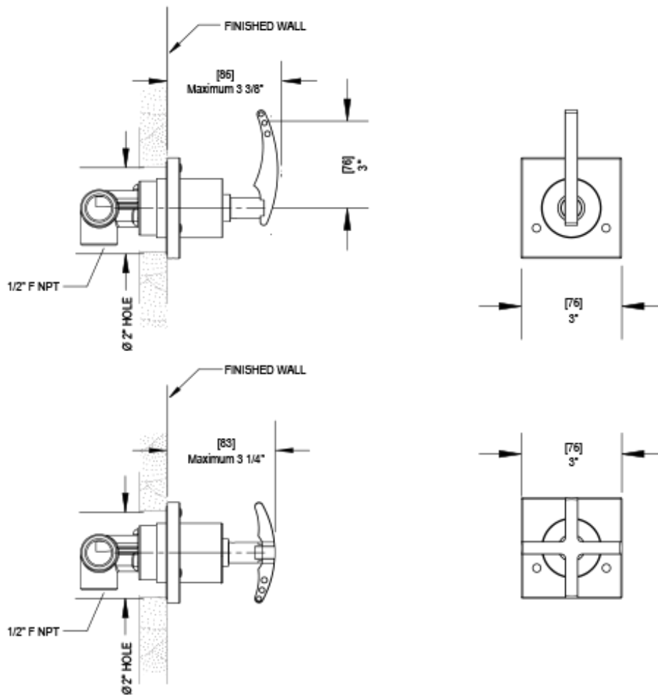
TWO WAY DIVERTER WITH SHUT-OFF
