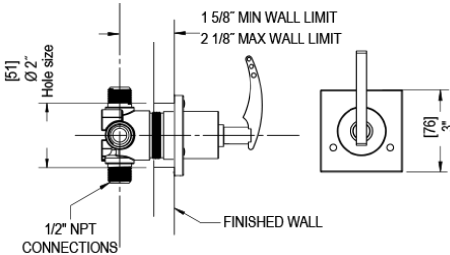
THREE WAY DIVERTER VALVE WITH SHARED OUTLETS IN BETWEEN FUNCTIONS
