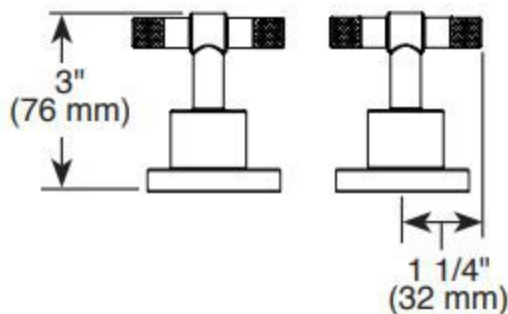
HL5339-▲ Wire Handle
