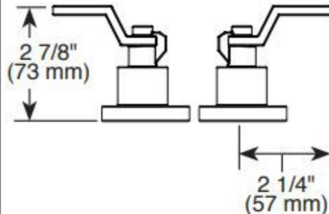
HW5332-▲ Wheel Handle
