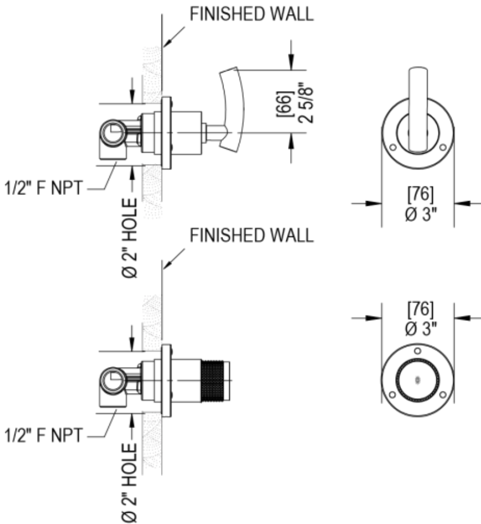
TWO WAY DIVERTER WITH SHUT-OFF
