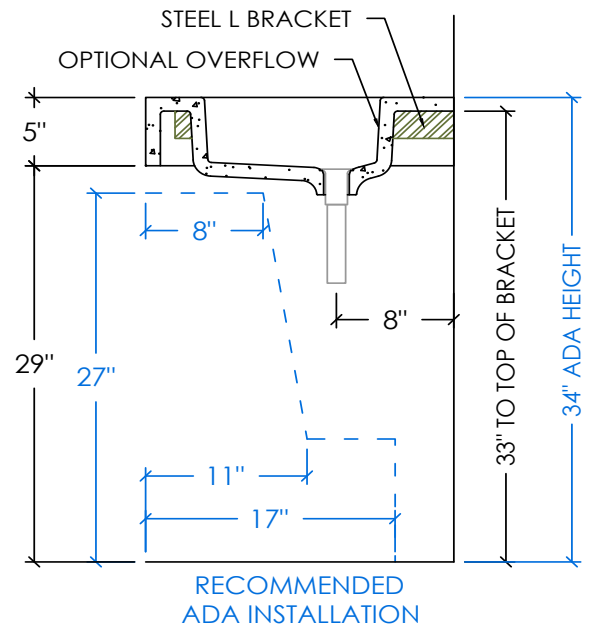
RIGHT SECTION
