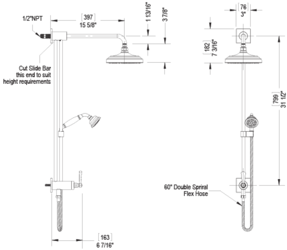
Critical Dimensions
