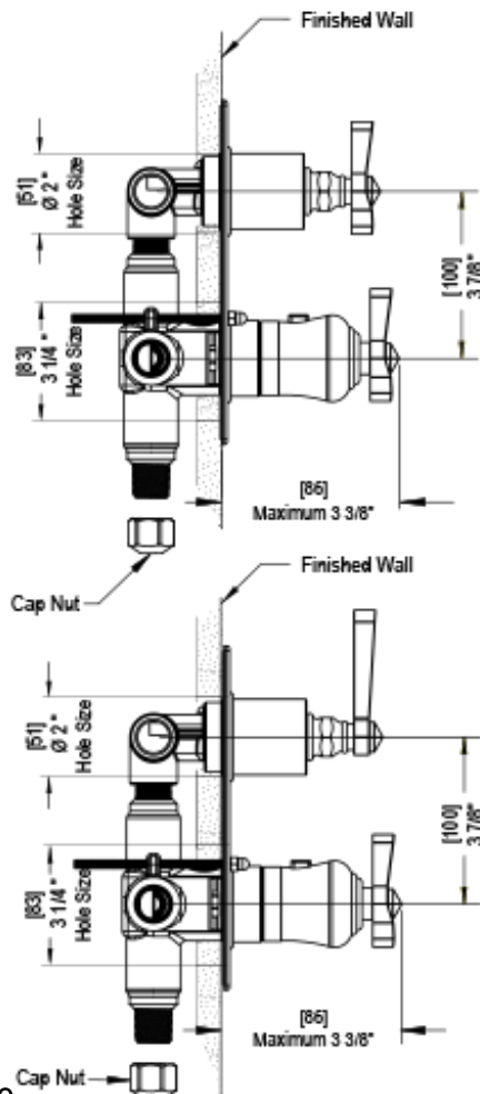
TEMPERATURE CONTROL VALVE WITH STOPS & TWO WAY DIVERTER WITH SHUT-OFF
