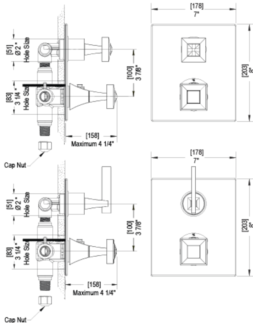
TEMPERATURE CONTROL VALVE WITH STOPS & TWO WAY DIVERTER WITH SHUT-OFF
