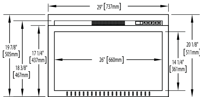
CEFB29H ILLUSTRÉE
