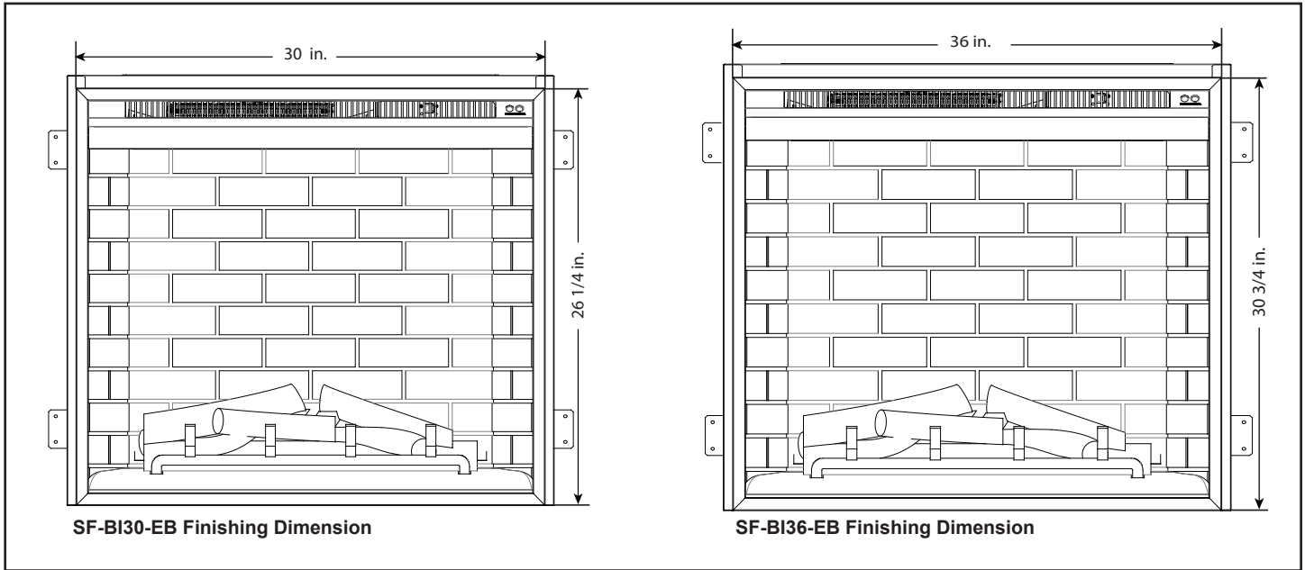
Figure 4.4 Finishing Dimensions
