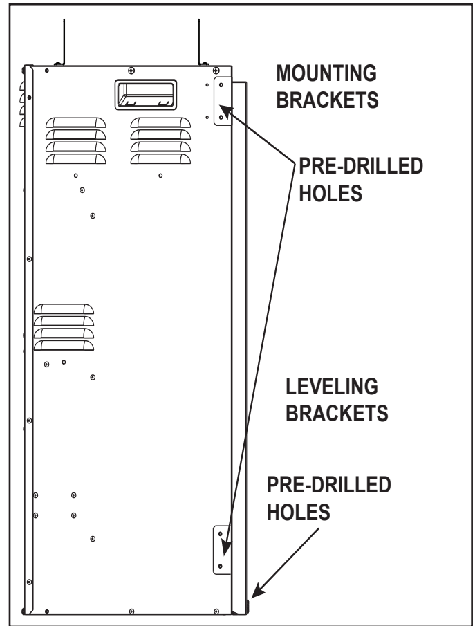
Figure 4.2 Pre-drilled Hole Locations
