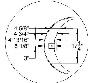
Faucet Deck Flat Dimensions
