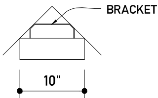
CORNER INSTALLATION (TOP VIEW)
