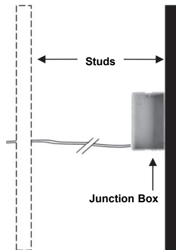
Figure 1. Location of ClearMirror wire leads and installing the junction box (Back View)
