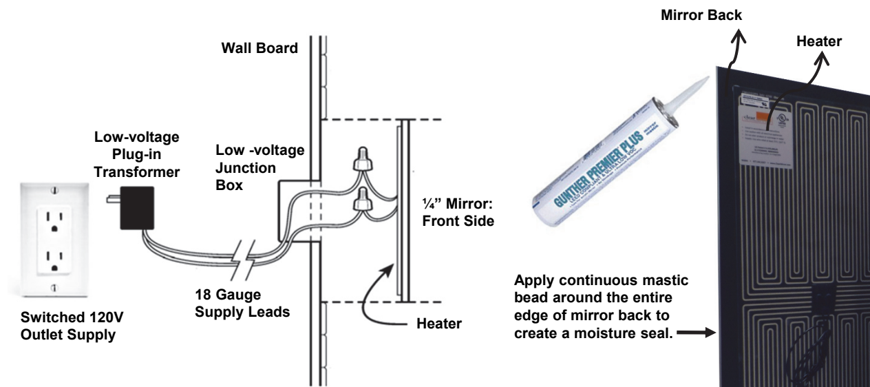
Figure 2. Connecting the wires and applying mirror mastic.
