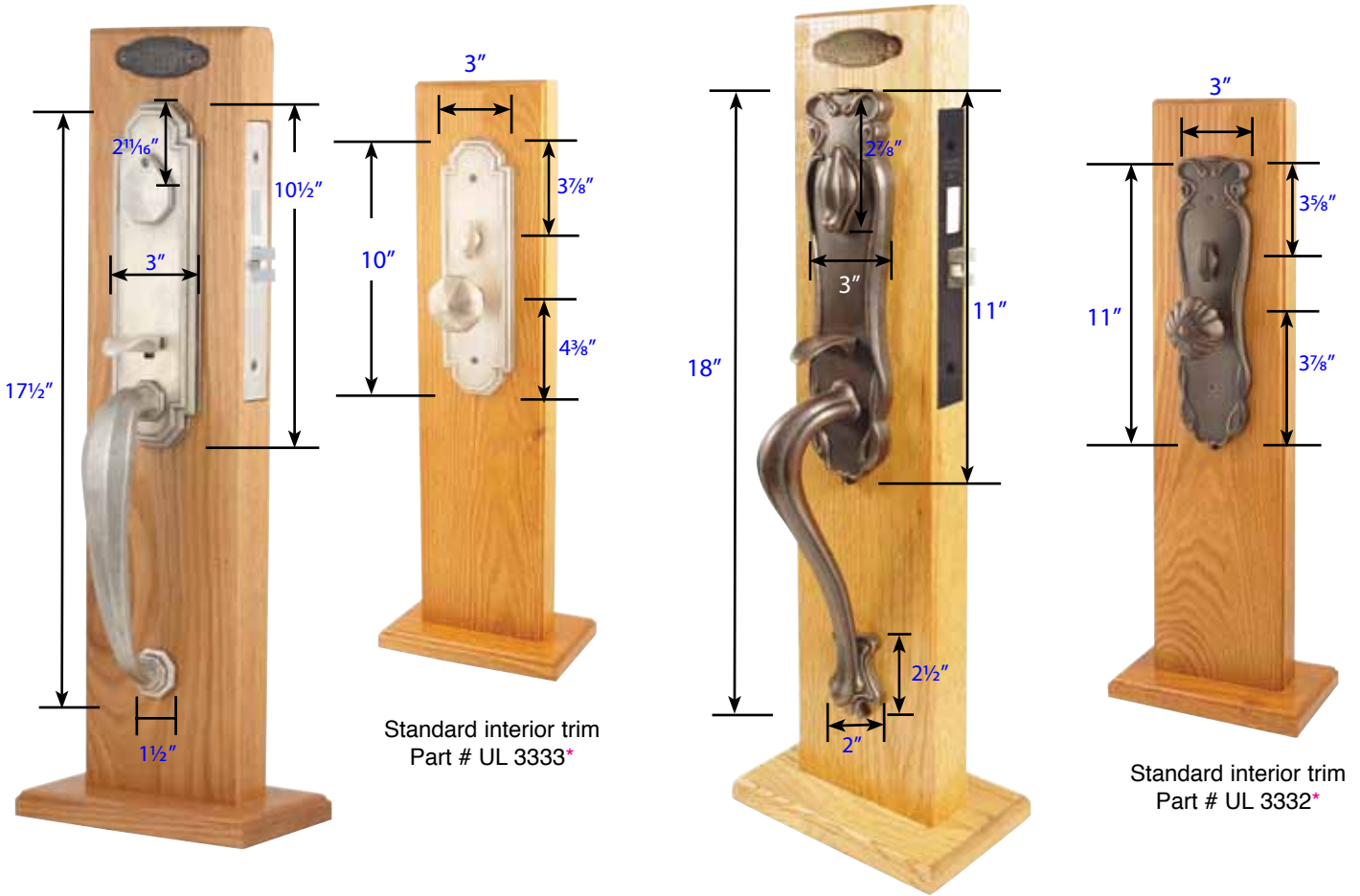
Octagon UL Mortise Entryset Part # UL 3333
