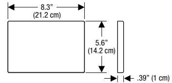
Omega Cover Plate for use with flush buttons
