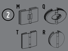
Glass-to-glass hinges
