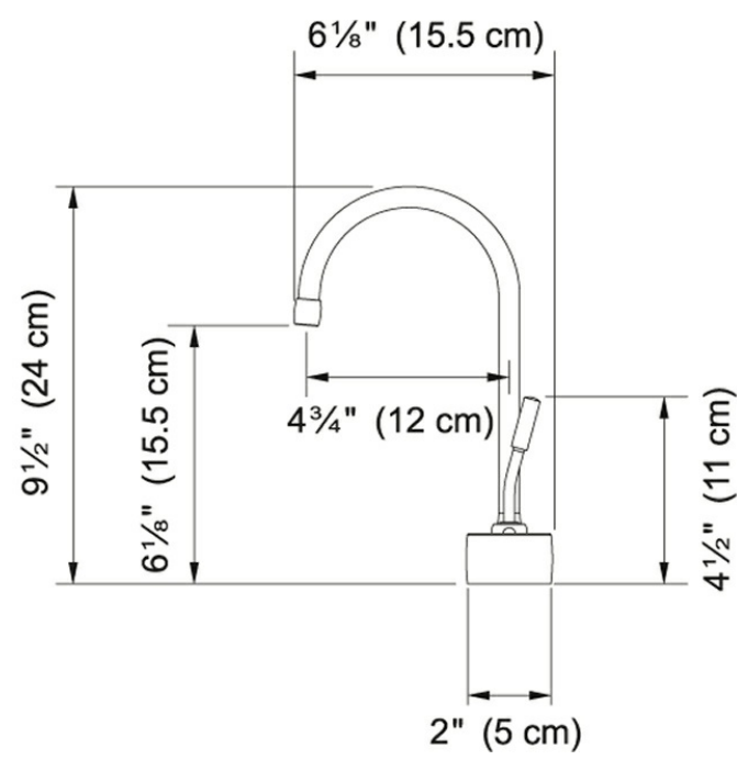
Technical Drawing
