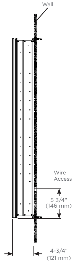
Surface Mount
