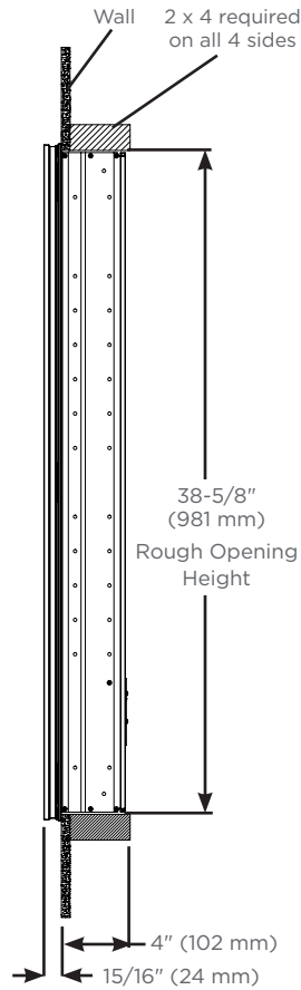
Recessed Mount
