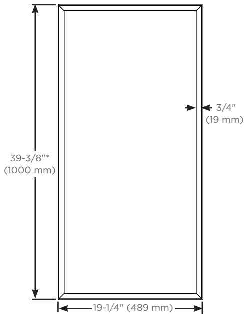
Cabinet Dimensions
