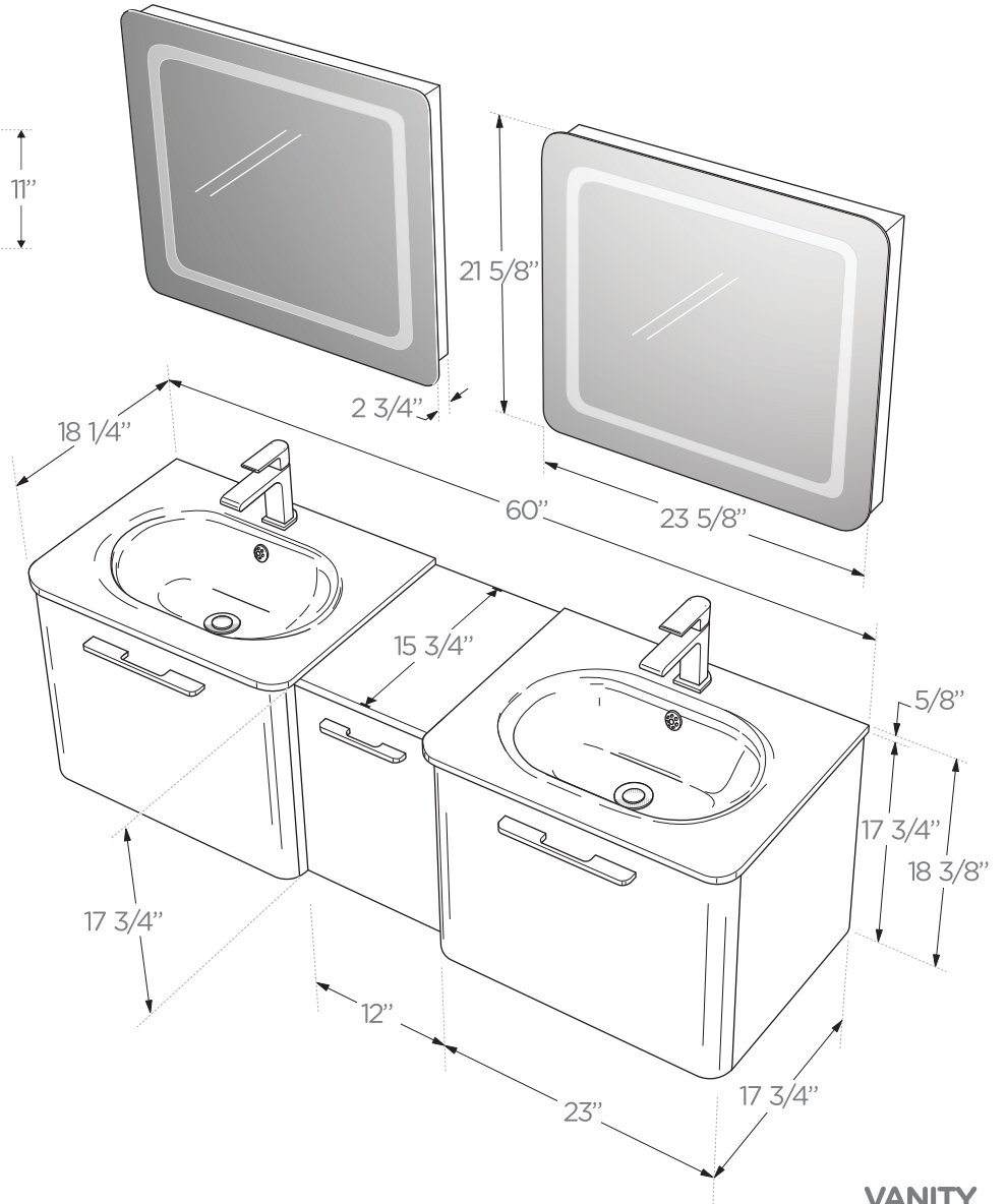
VANITY front view
